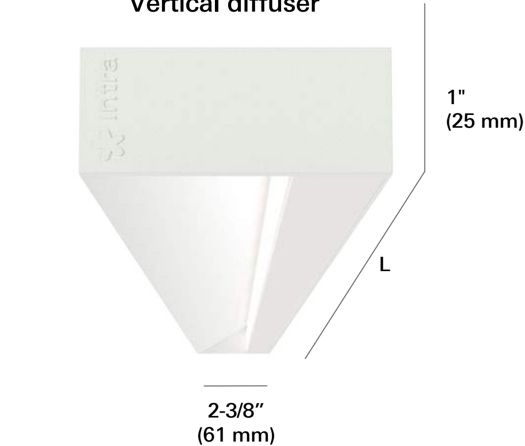
Cove 25 V Vertical diffuser
